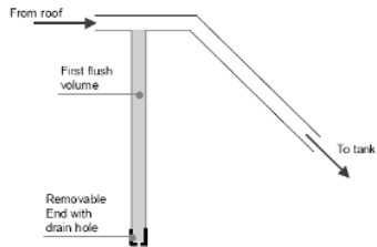
Figure 10 Simple first-flush diverter
