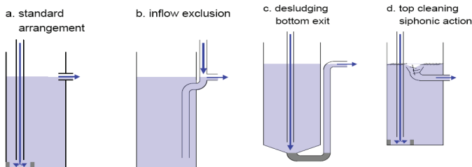
Figure 24 Design configurations for tank overflows. Source: South Pacific Applied Geoscience Commission (2004)
