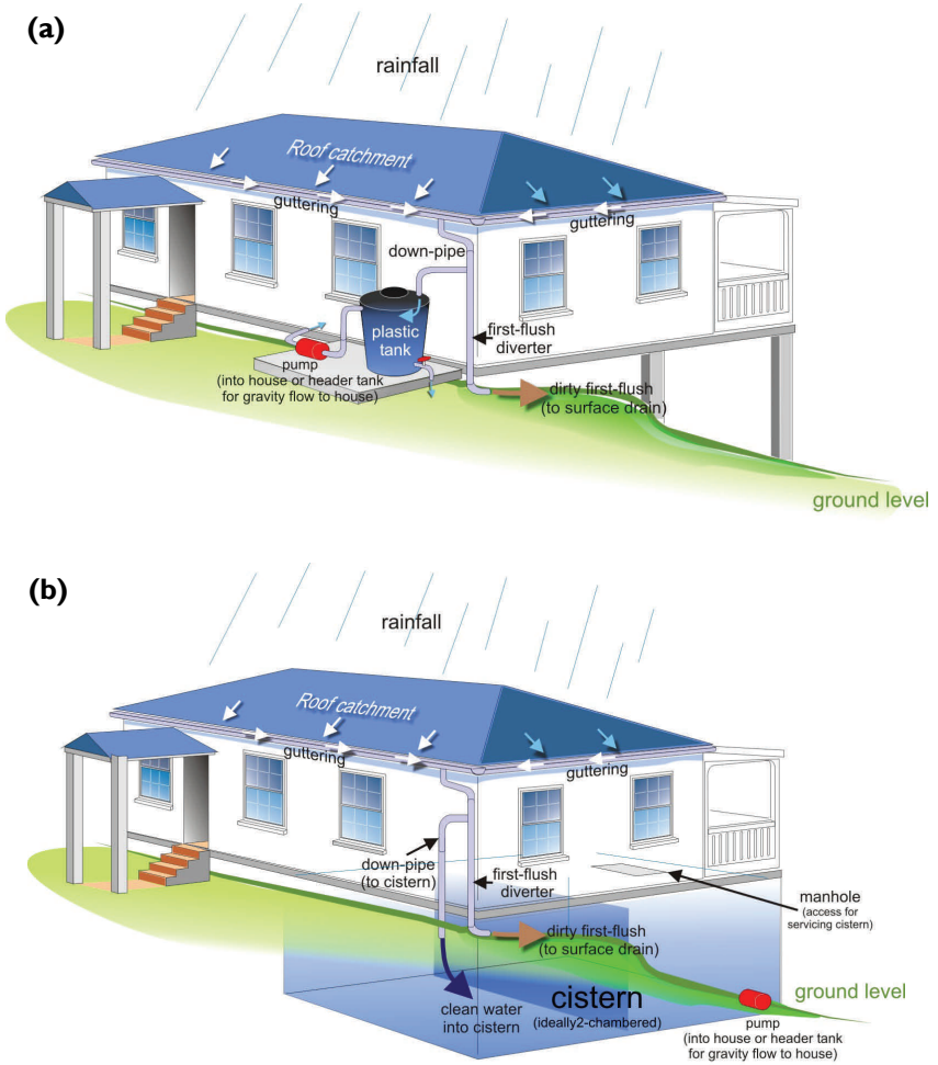
Figure 7 Typical domestic RWH systems with (a) above-ground and (b) below-ground storage
