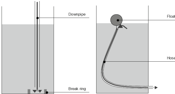
Figure 23 Design configurations for (a) tank inflow and (b) outflow. Source: South Pacific Applied Geoscience Commission (2004)
