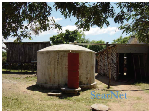
Figure 19 Typical ferrocement tank
