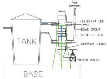
Figure 13 Upflow filter design. Used in UNEP/CEHI RWH project in Antigua and Barbuda (Design by Hastin Barnes, Antigua and Barbuda Public Utilities Authority)
