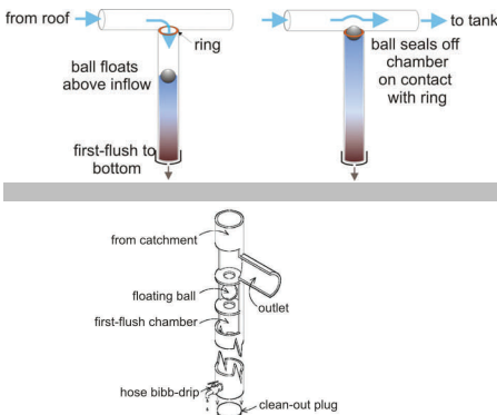
Figure 12 Examples of first-flush systems using float-ball mechanism
