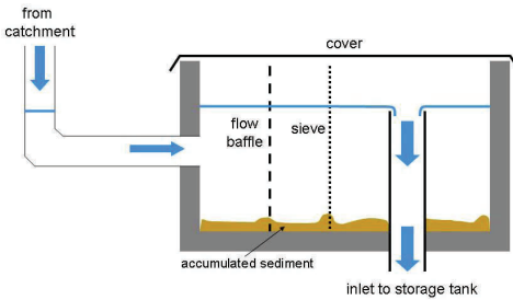
Figure 17 Baffle tank design to trap debris
