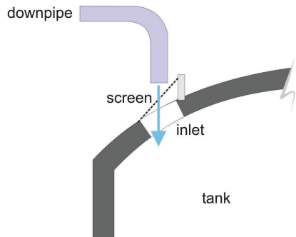
Figure 16 Design configuration for a self-cleaning screen
