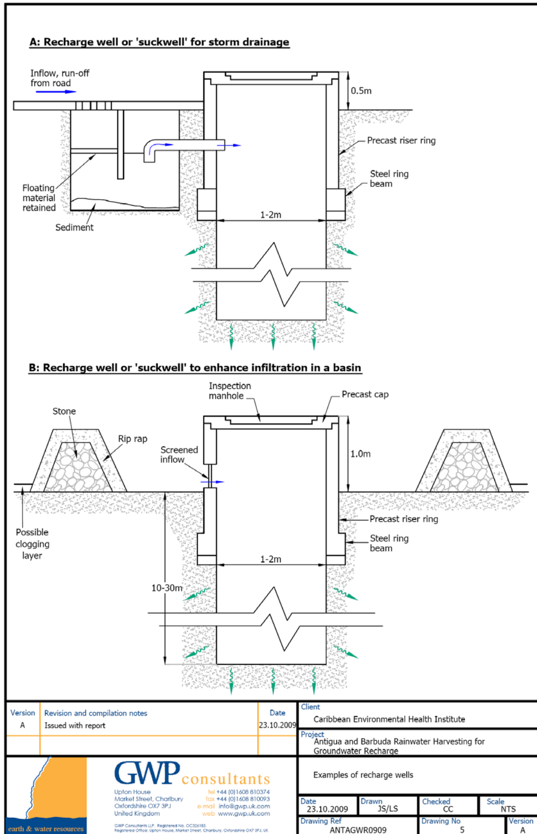
Drawing 5: Example of recharge wells/shafts
